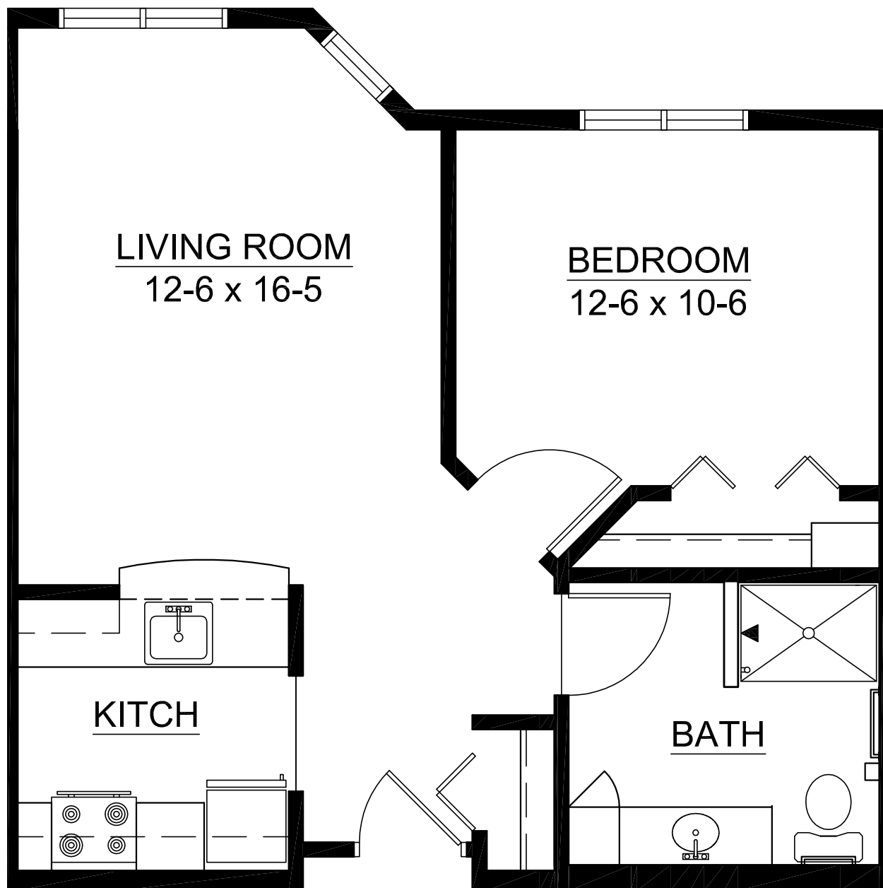
B1-unit One Bedroom 625 s.f.
